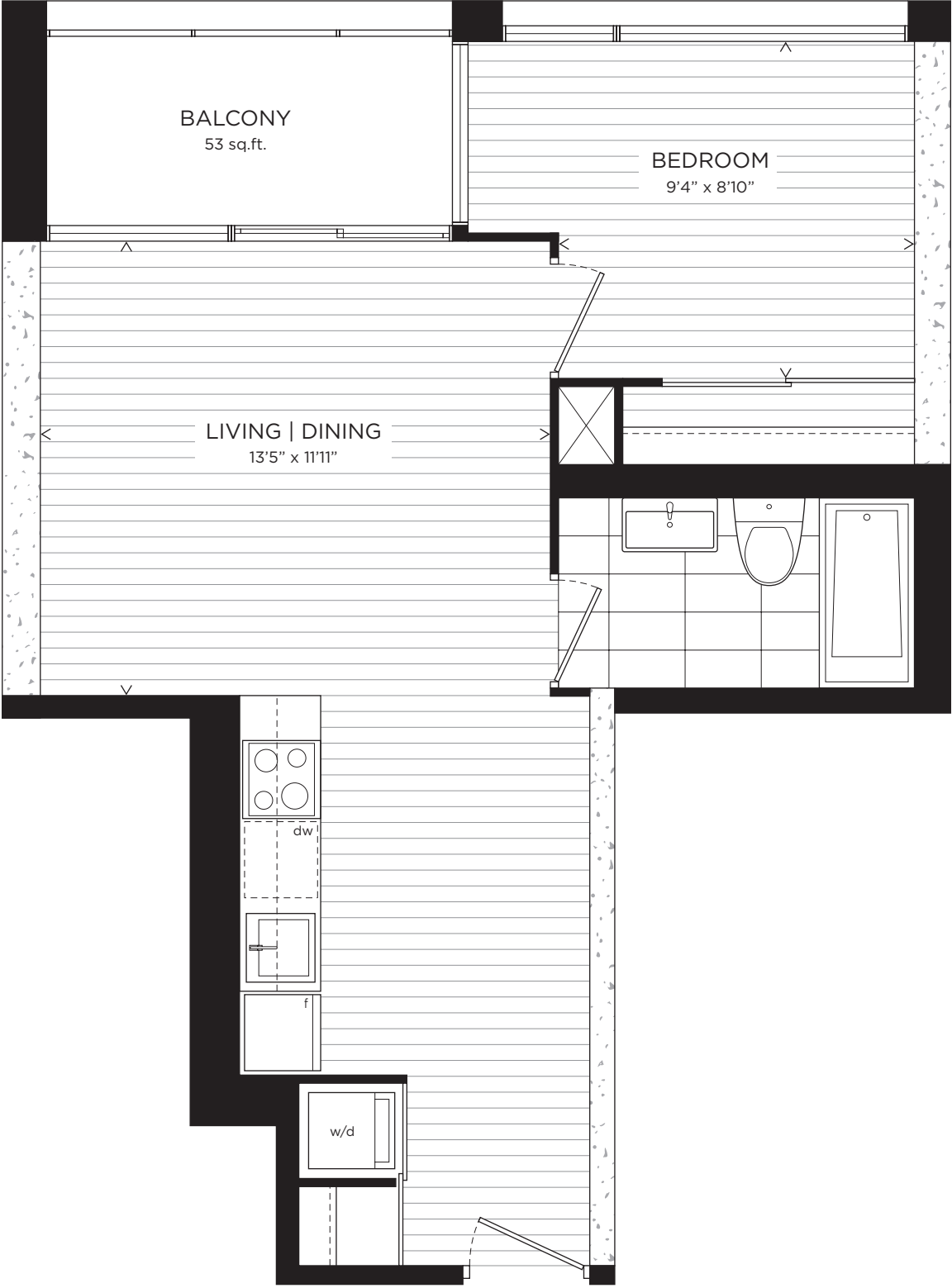
LEVEL 2
